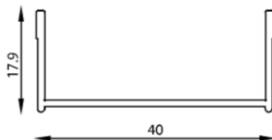
1202 Jamba
