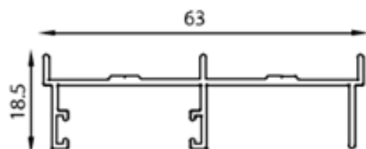
2009 Jamba
