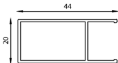
2017 Batiente Termopanel
